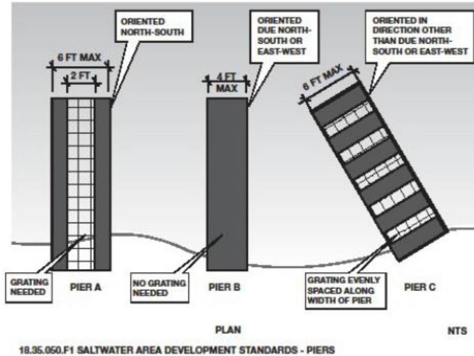
FIGURE 9 – PIER STANDARDS
