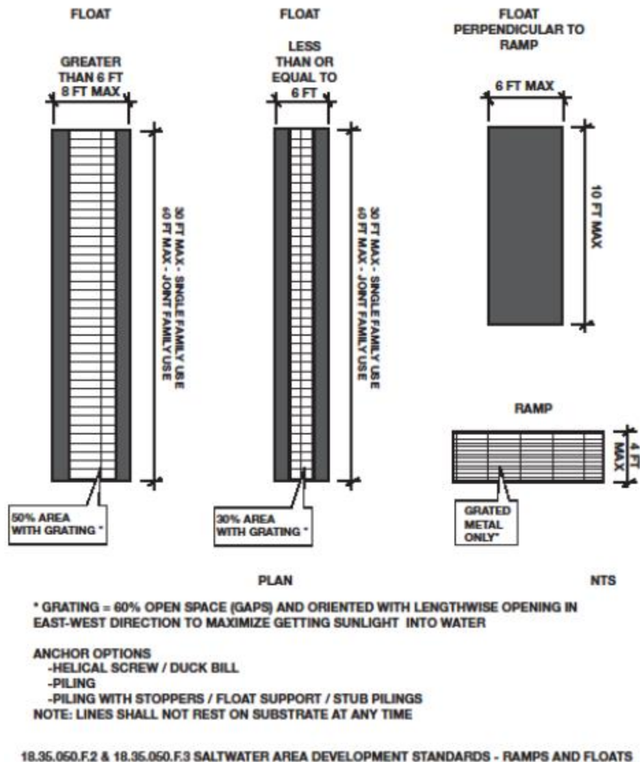
FIGURE 10 – FLOAT AND RAMP STANDARDS
